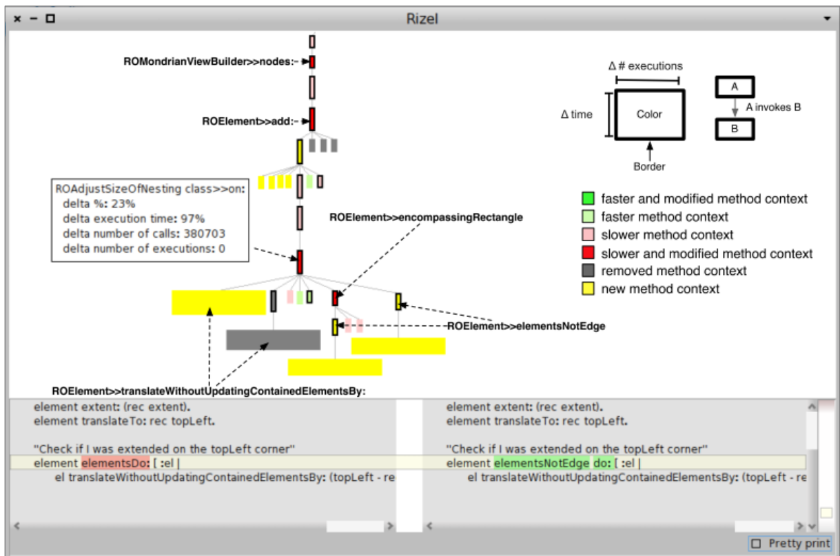
Figura 50: Exemplo do Performance Evolution Blueprint [14].
