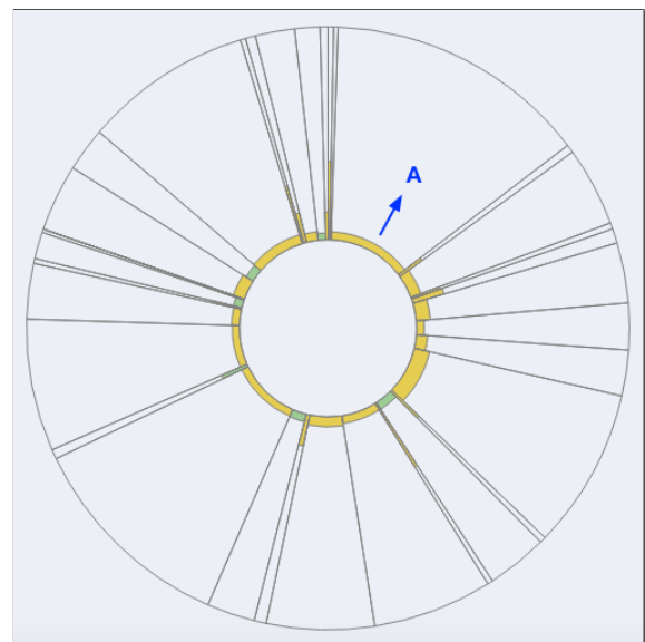
(b) Jetty, 9.3.16/9.4.0.
