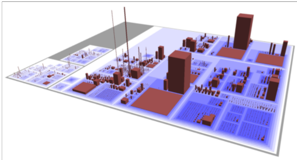
Figura 4: Codecity [58].
