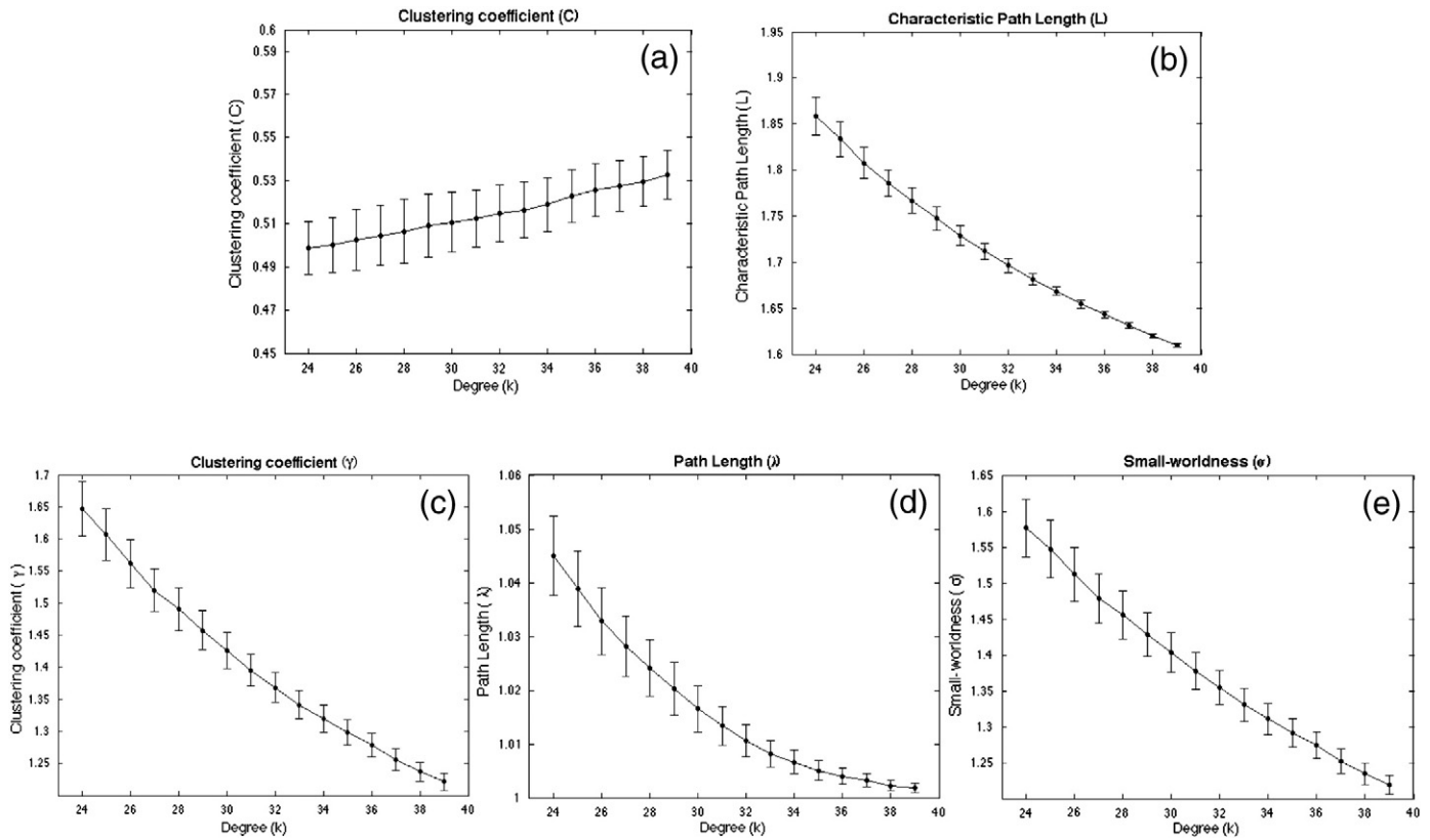
Fig. 7. Examples of topological measures. (a) Clustering coefficient ( C ), (b) characteristic path length ( L ), (c) normalized clustering coefficient ( \gamma = C/C_{\text{rand}} ), (d) normalized path length ( \lambda = L/L_{\text{rand}} ), and (e) small-worldness ( \sigma = \gamma/\lambda ). Metrics were calculated for a healthy group (7 subjects) as a function of the degree k . Error bars indicate standard error of the mean.
