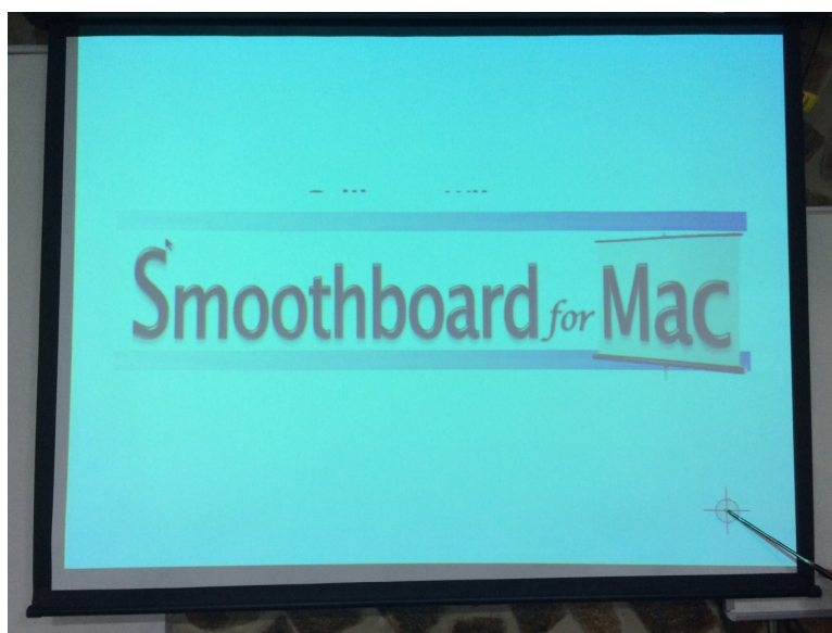
Figura 4.6: Software Smoothboard.
