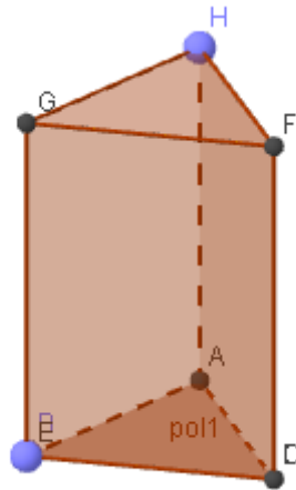
Figura 3.9: Prisma triangular
