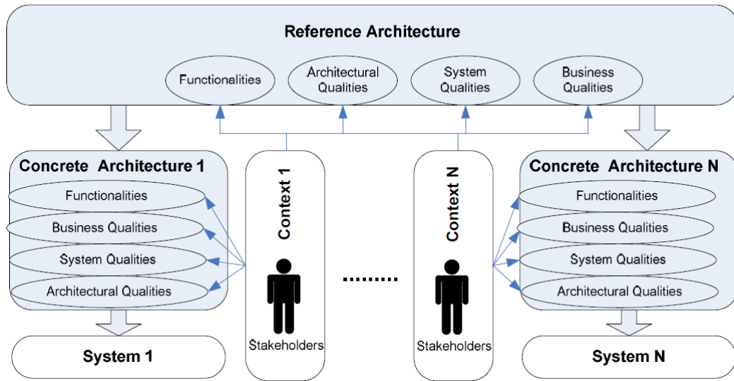
Figure 5: The role of stakeholders and contexts for reference and concrete architectures (ANGELOV; TRIENEKENS; GREFFEN, 2008).
