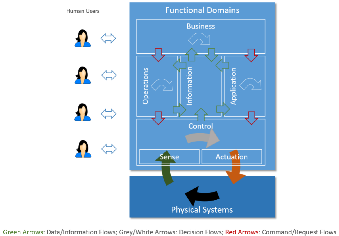
Figure 11: IIRA Functional Domains (LIN; CRAWFORD; MELLOR, 2017).
