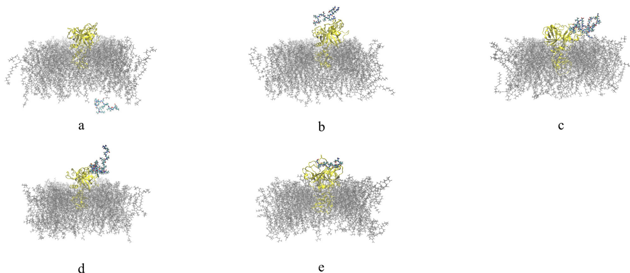
Fig. 6 Final structural analysis of the interaction between theoretical models of analogous peptides obtained by cleavage of TTIp 56/287 with TMRSS2. a: ID 32 – Peptide analogue to Pep1; b: ID 76 – Peptide analogue to Pep2; c: ID 63 – Peptide analogue to Tryp1; d: ID 336 – Peptide analogue to Tryp2; e: ID 101 – Peptide analogue to Chym1. TTIp 56/287: trypsin inhibitor purified from tamarind seeds (TTIp), model number 56, in conformation number 287. TMRSS2: transmembrane serine protease 2.
