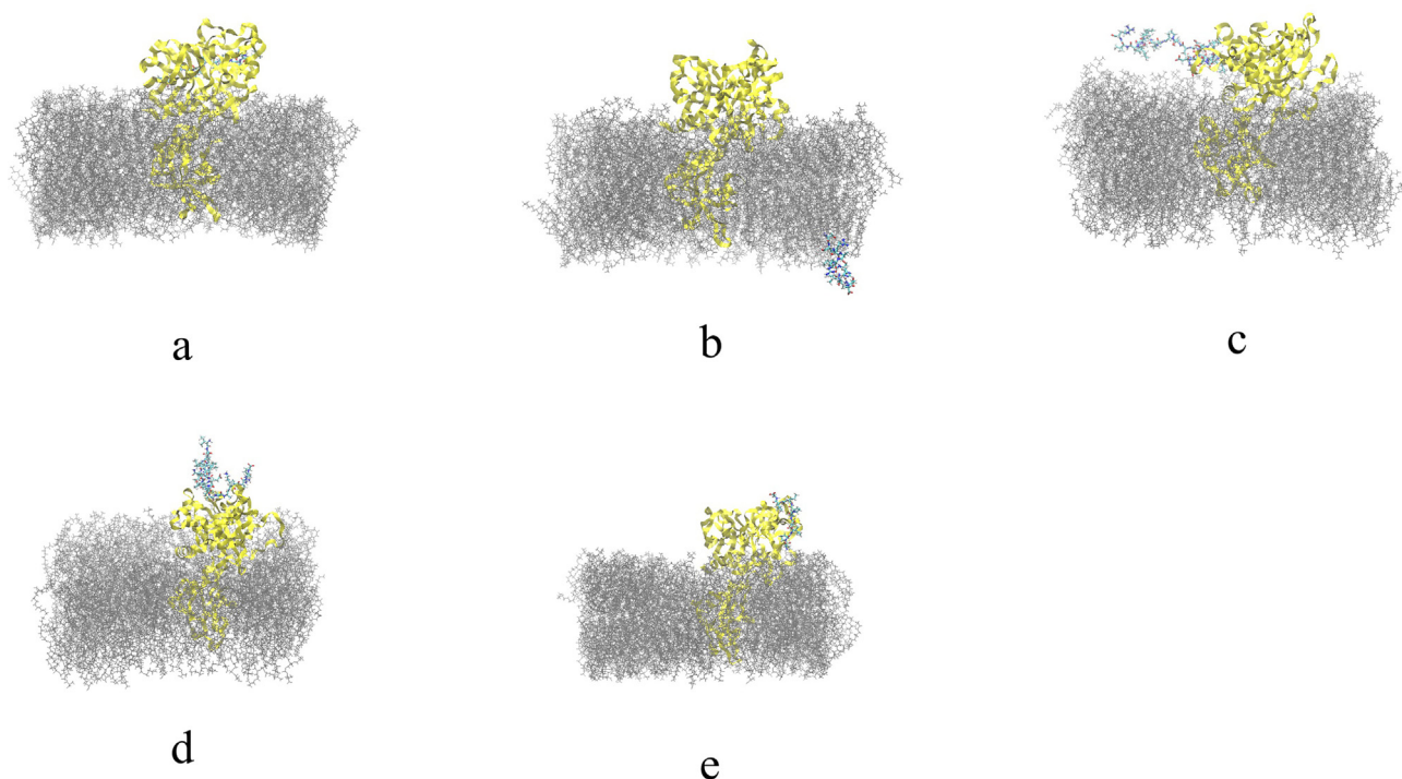
Fig. 5 Final structural analysis of the interaction between theoretical models of native peptides obtained by cleavage of TTIp 56/287 with TMRSS2. a: Pep1 – Peptide obtained by cleavage with pepsin; b: Pep2 – Peptide obtained by cleavage with pepsin; c: Tryp1 – Peptide obtained by cleavage with trypsin; d: Tryp2 – Peptide obtained by cleavage with trypsin; e: Chym1 – Peptide obtained by cleavage with chymotrypsin. TTIp 56/287: trypsin inhibitor purified from tamarind seeds (TTIp), model number 56, in conformation number 287. TMRSS2: transmembrane serine protease 2.
