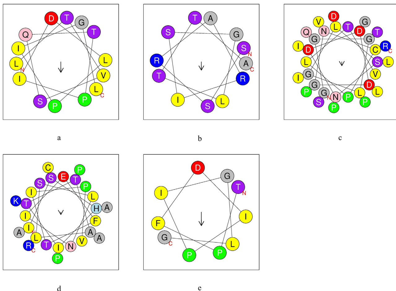
Fig. 4 \alpha -helix structure of analogous peptides obtained by cleavage of TTIp 56/287. a: ID 32 – Peptide analogue to Pep1; b: ID 76 – Peptide analogue to Pep2; c: ID 63 – Peptide analogue to Tryp1; d: ID 336 – Peptide analogue to Tryp2; e: ID 101 – Peptide analogue to Chym1. Yellow – hydrophobic residues; purple – serine and threonine residues; dark blue – basic residues; red – acid residues; pink – asparagine and glutamine residues; gray – alanine and glycine residues; light blue – histidine residues; green – proline residues. TTIp 56/287: trypsin inhibitor purified from tamarind seeds (TTIp), model number 56, in conformation number 287.
