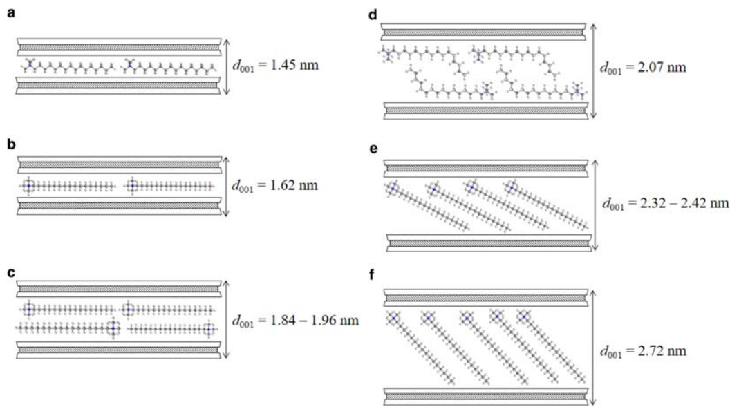
FIG. 6. Orientations of alkylammonium ions in the basal spacing of silicates: (a) monolayer with perpendicular conformation; (b) monolayer with parallel conformation; (c) bilayer; (d) pseudotrilayer; and (e,f) paraffin-type arrangements of alkylammonium ions with different tilting angles of the alkyl chains.
